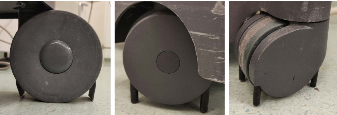
Figure 1: Wheels of mobile X-ray machines, showing cable deflectors, at front and back of all castors, and reaching fully to the ground.
